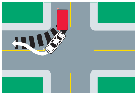
Turning right when towing a trailer - note the path of vehicle and trailer wheels.
